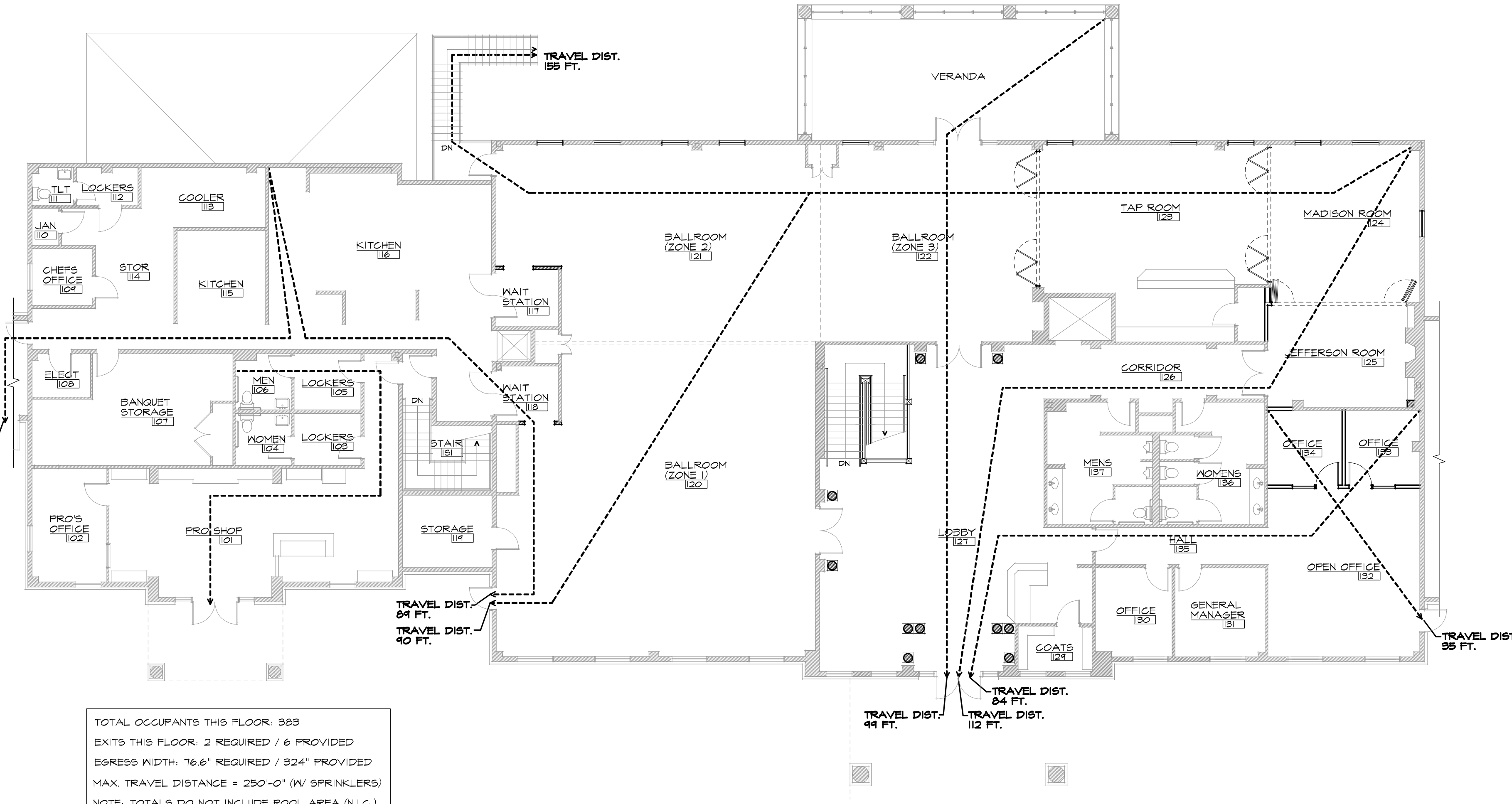
2 MAIN FLOOR LIFE SAFETY PLAN
