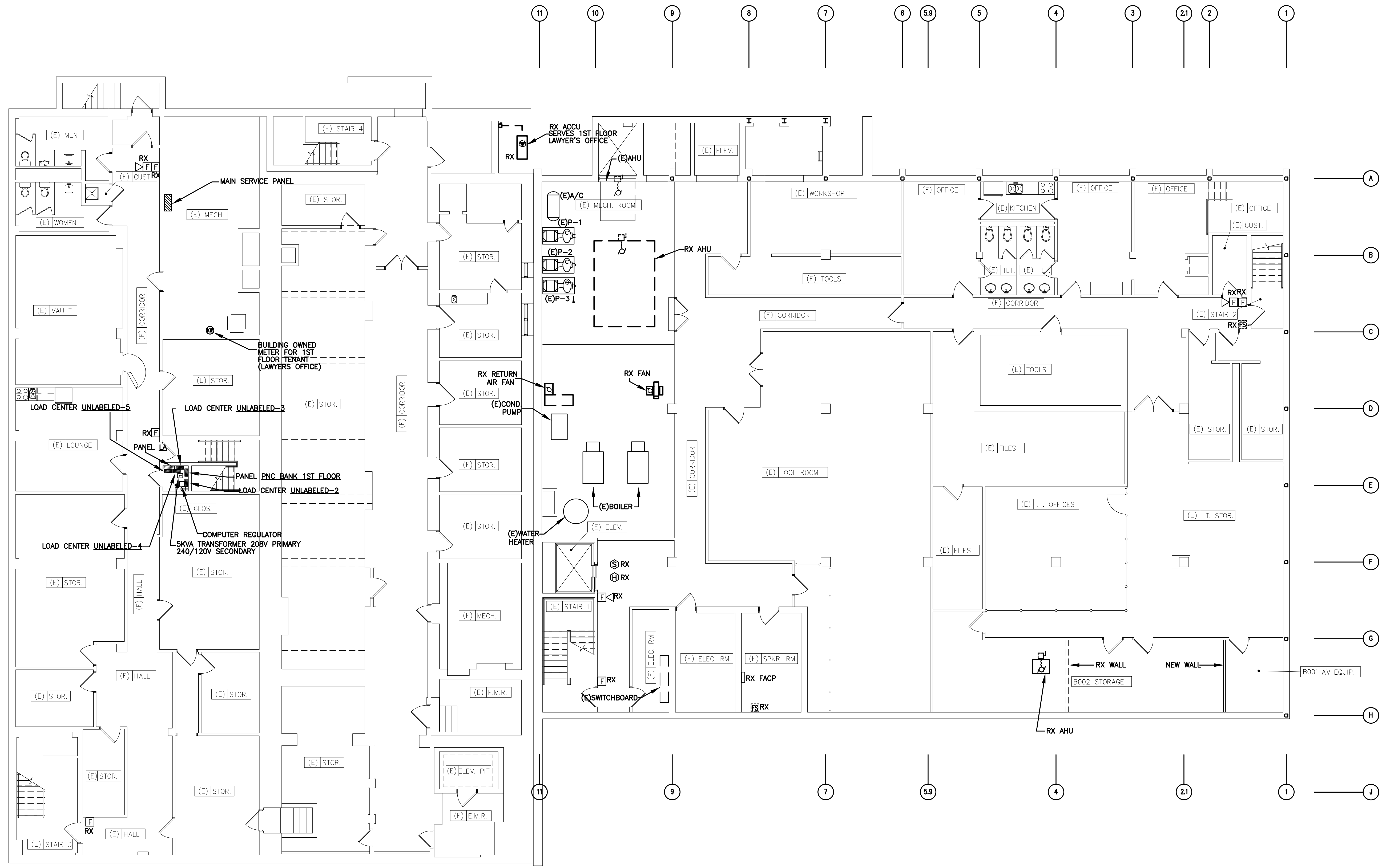
BASEMENT FLOOR PLAN - ELECTRICAL DEMO SCALE: 1/8" = 1'-0"
