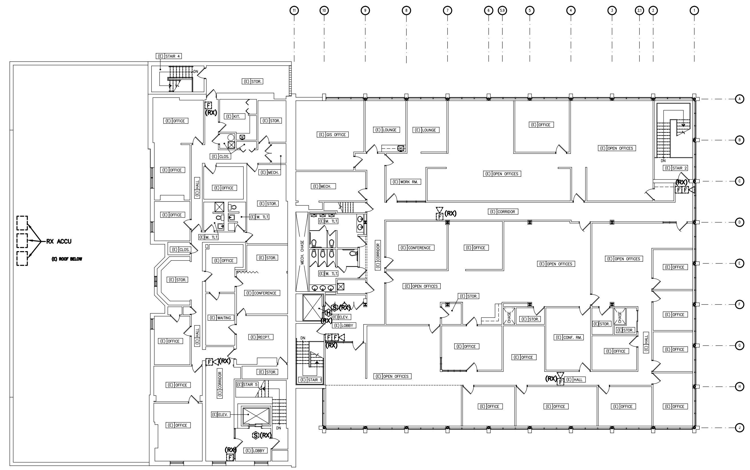
THIRD FLOOR PLAN - ELECTRICAL DEMO SCALE: 1/16" = 1'-0"
