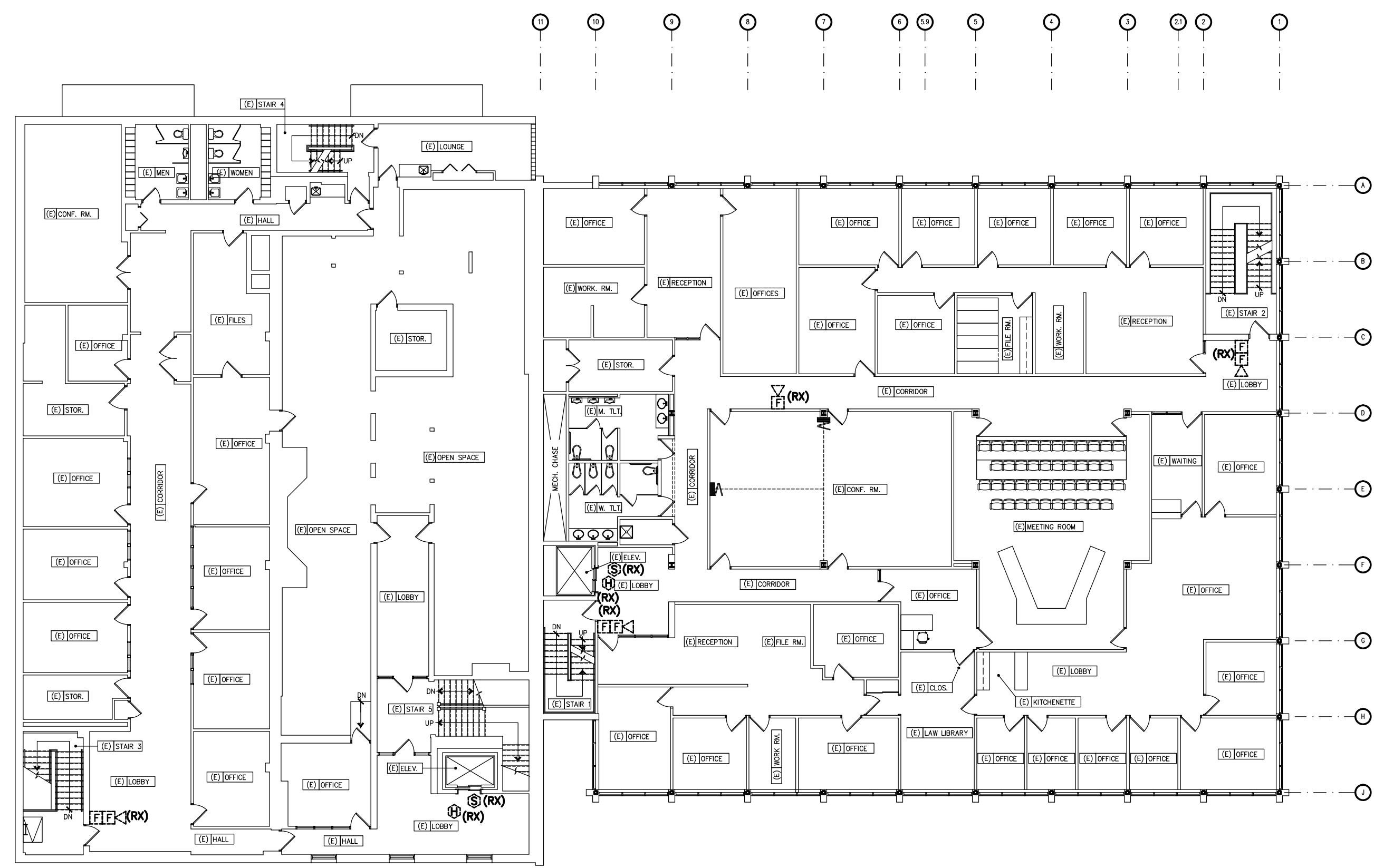
SECOND FLOOR PLAN - ELECTRICAL DEMO SCALE: 1/16" = 1'-0"
