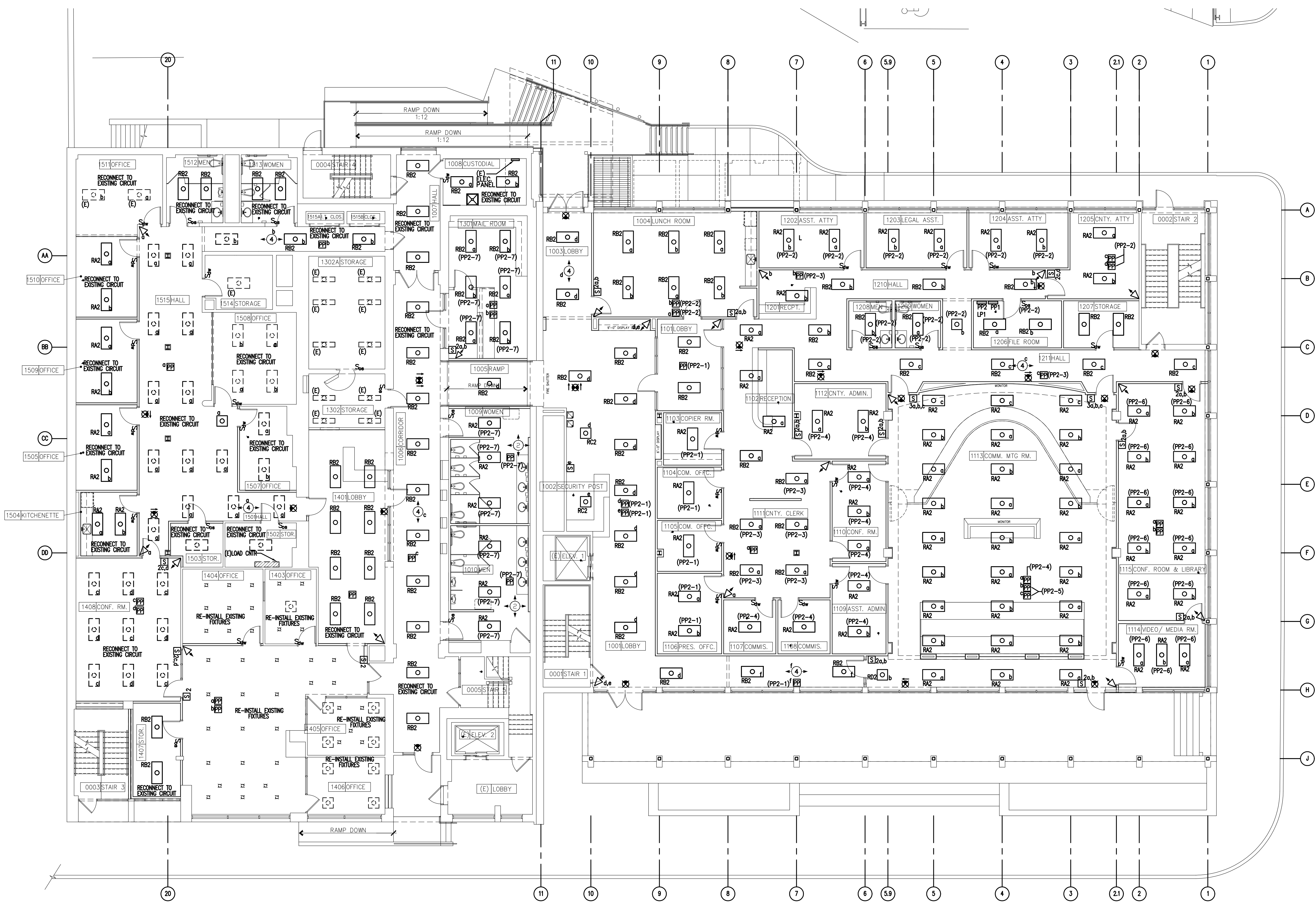
FIRST FLOOR PLAN - LIGHTING SCALE: 1/8" = 1'-0"
