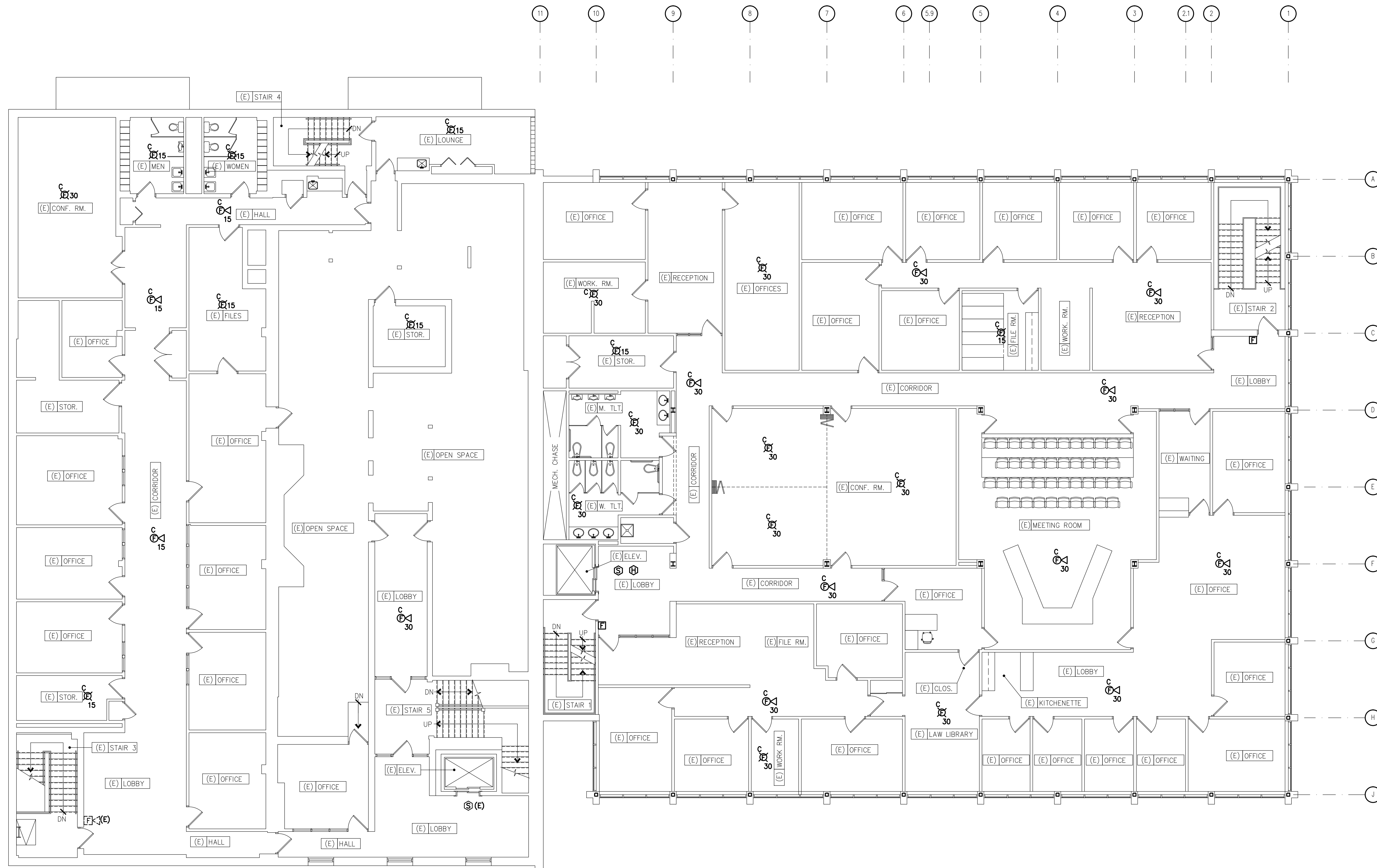
SECOND FLOOR PLAN - FIRE ALARM - NEW SCALE: 1/8" = 1'-0"
