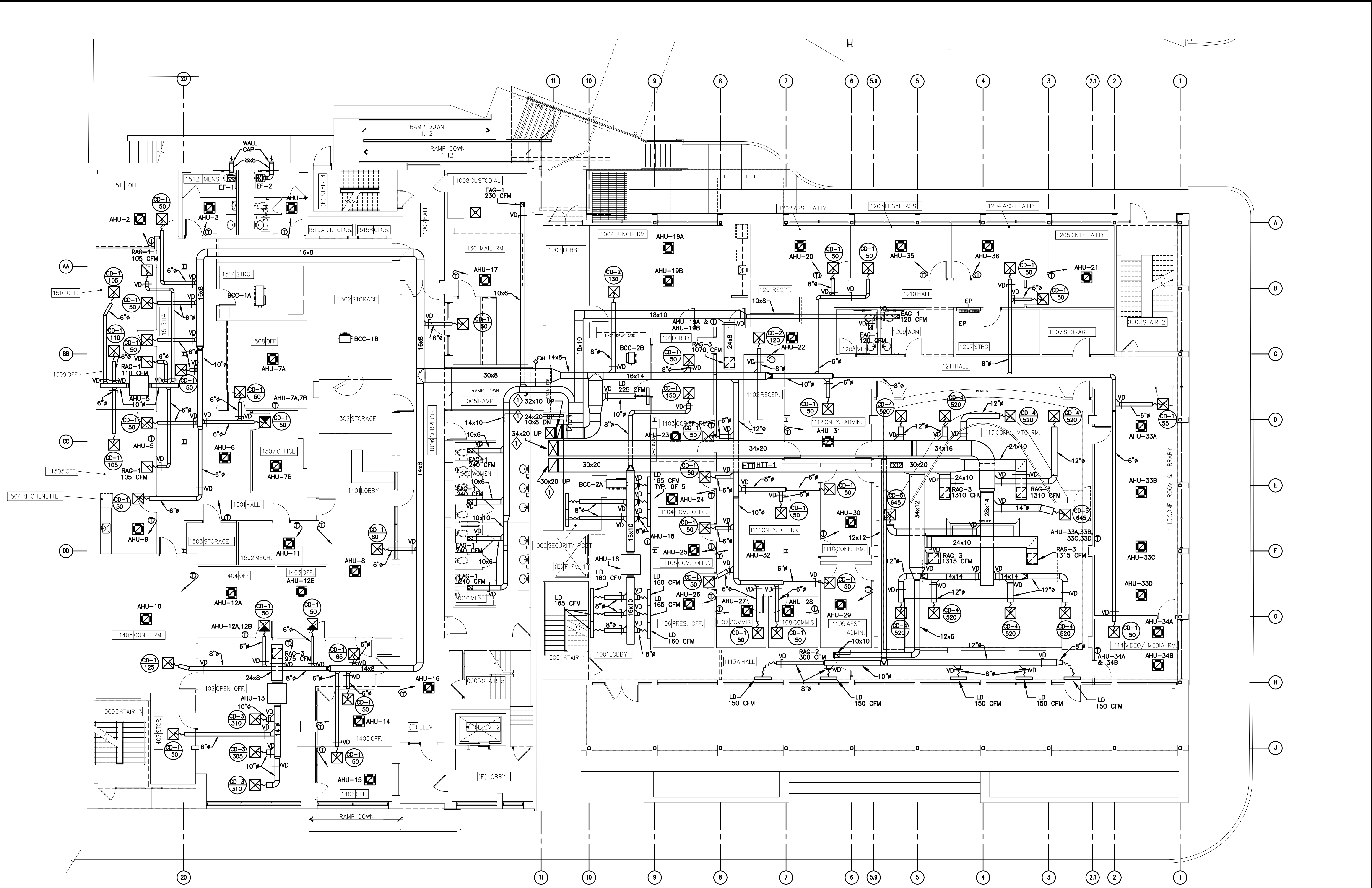
FIRST FLOOR PLAN - HVAC NEW SCALE: 1/8" = 1'-0"
