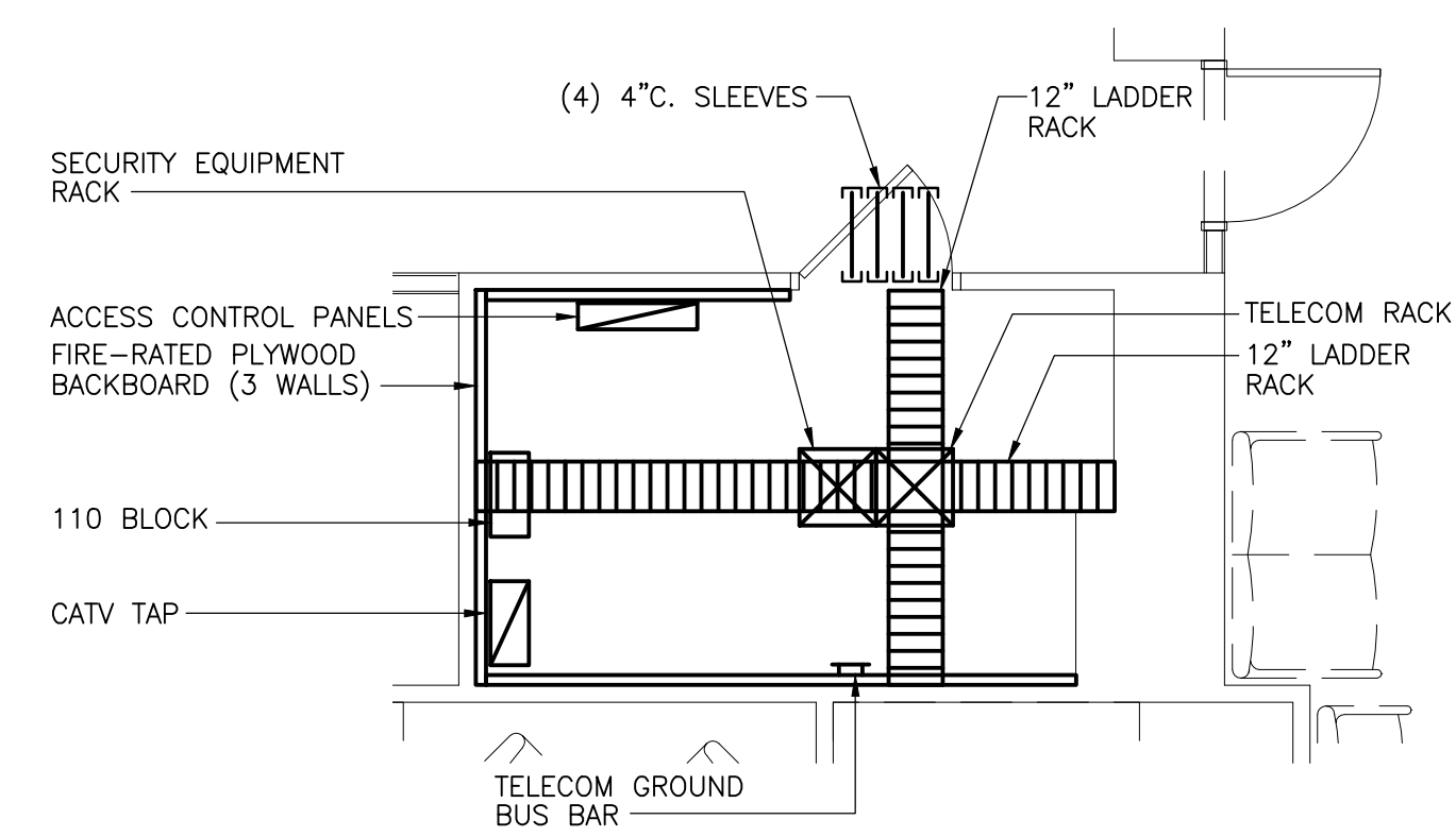
FIRST FLOOR PART PLAN - IDF ROOM 1502 SCALE: 1/4" = 1'-0"
