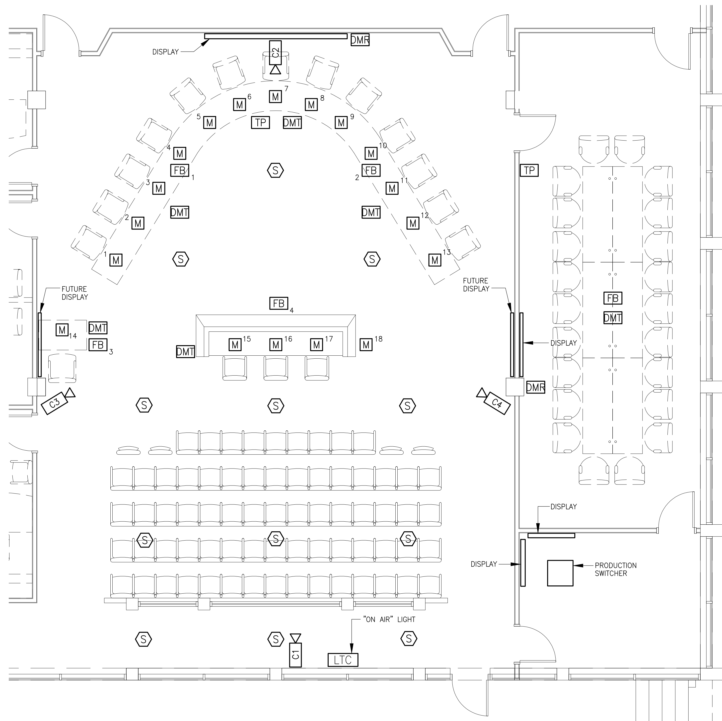
FIRST FLOOR PART PLAN - AUDIO/VIDEO SCALE: 1/4" = 1'-0"
