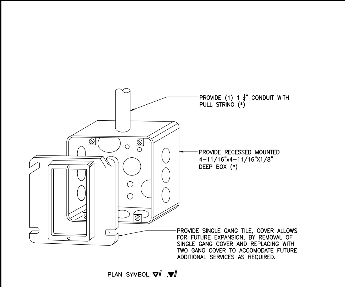
3 COMMUNICATIONS OUTLET DETAIL
