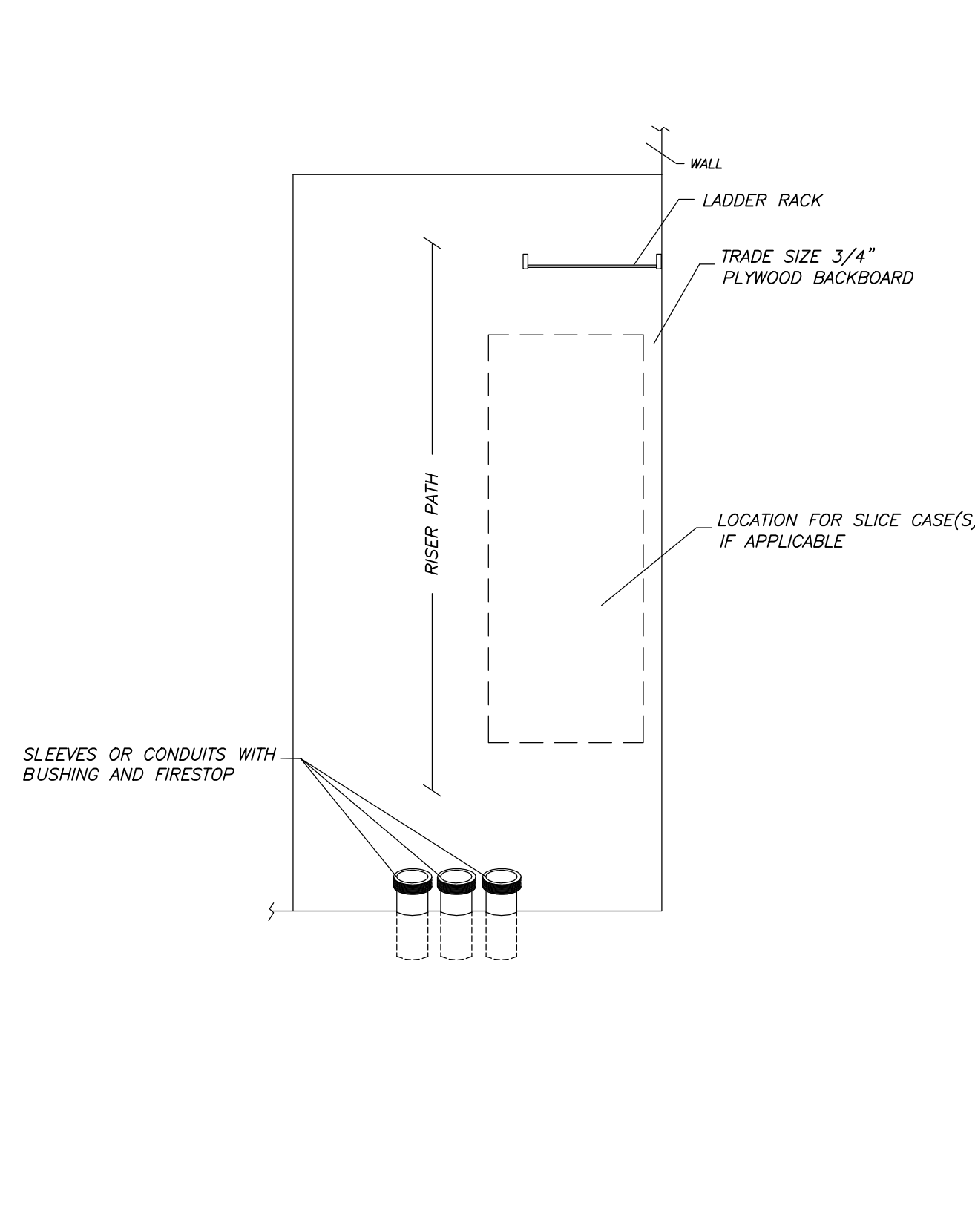
6 RISER BACKBOARD ELEVATION
