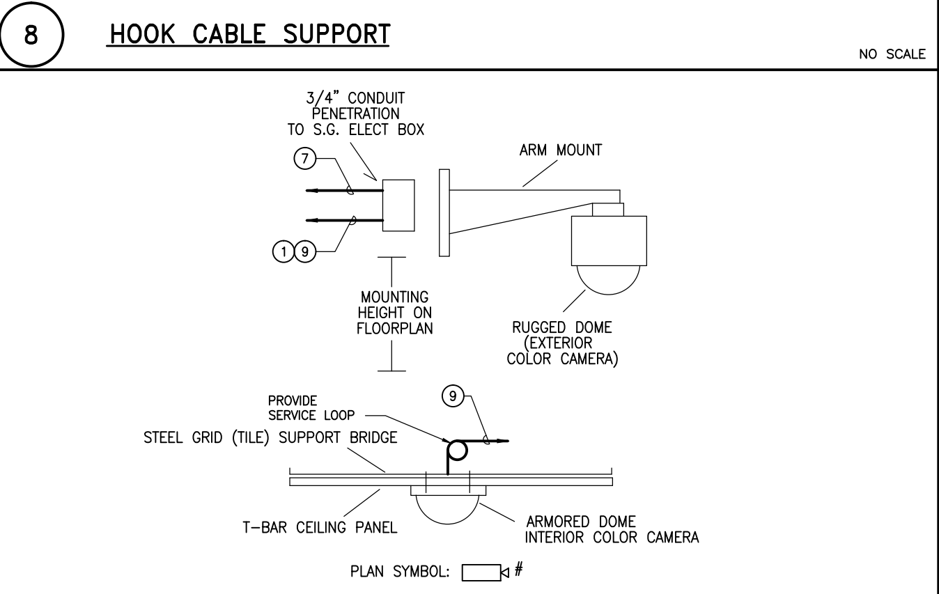
10 TYP. CCTV CAMERA MOUNTING DETAILS
