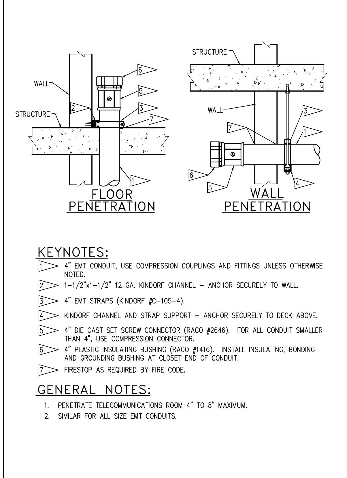
5 RISER CONDUIT END FITTINGS DETAIL
