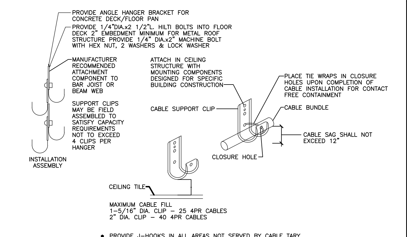
8 HOOK CABLE SUPPORT
