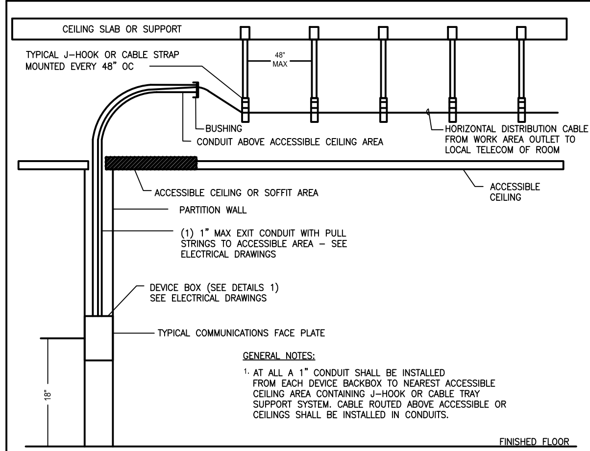
1 TYPICAL WALL MOUNTED OUTLET DEVICE BOX
