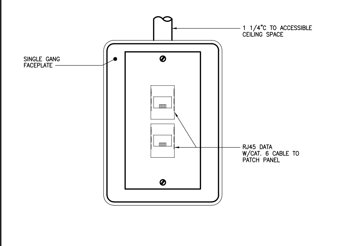
7 TYPICAL DUAL OUTLET
