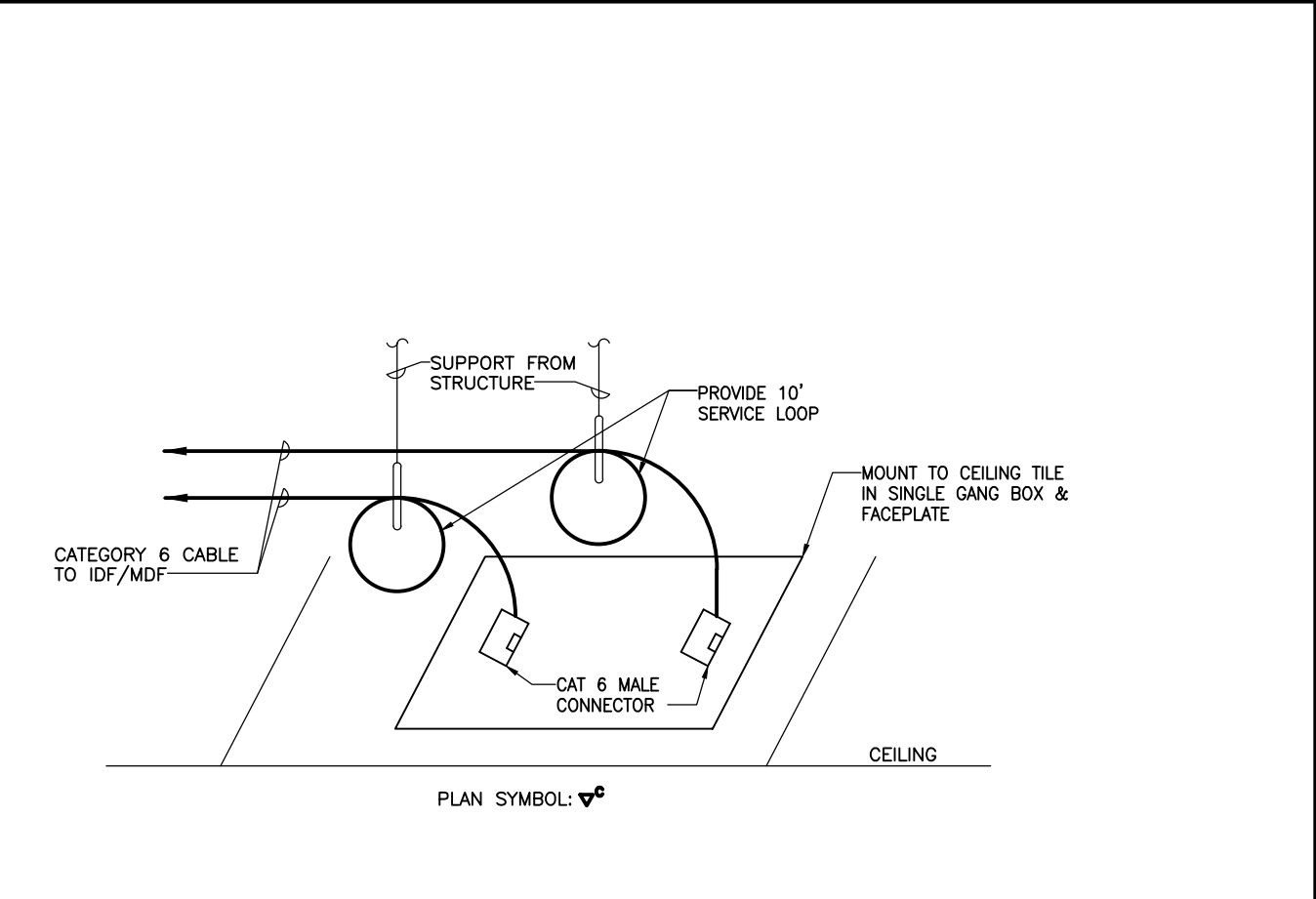
4 WIRELESS ACCESS CONNECTION DETAIL
