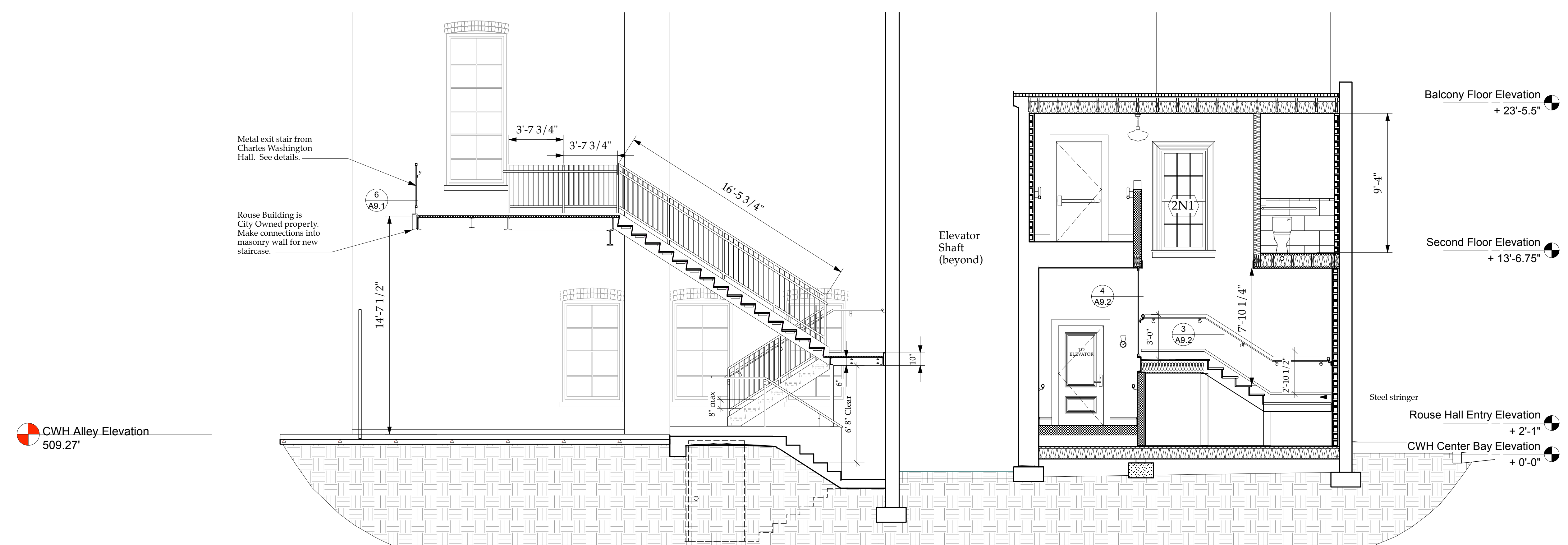
2 Building Section D Scale: 1/4" = 1'-0"
