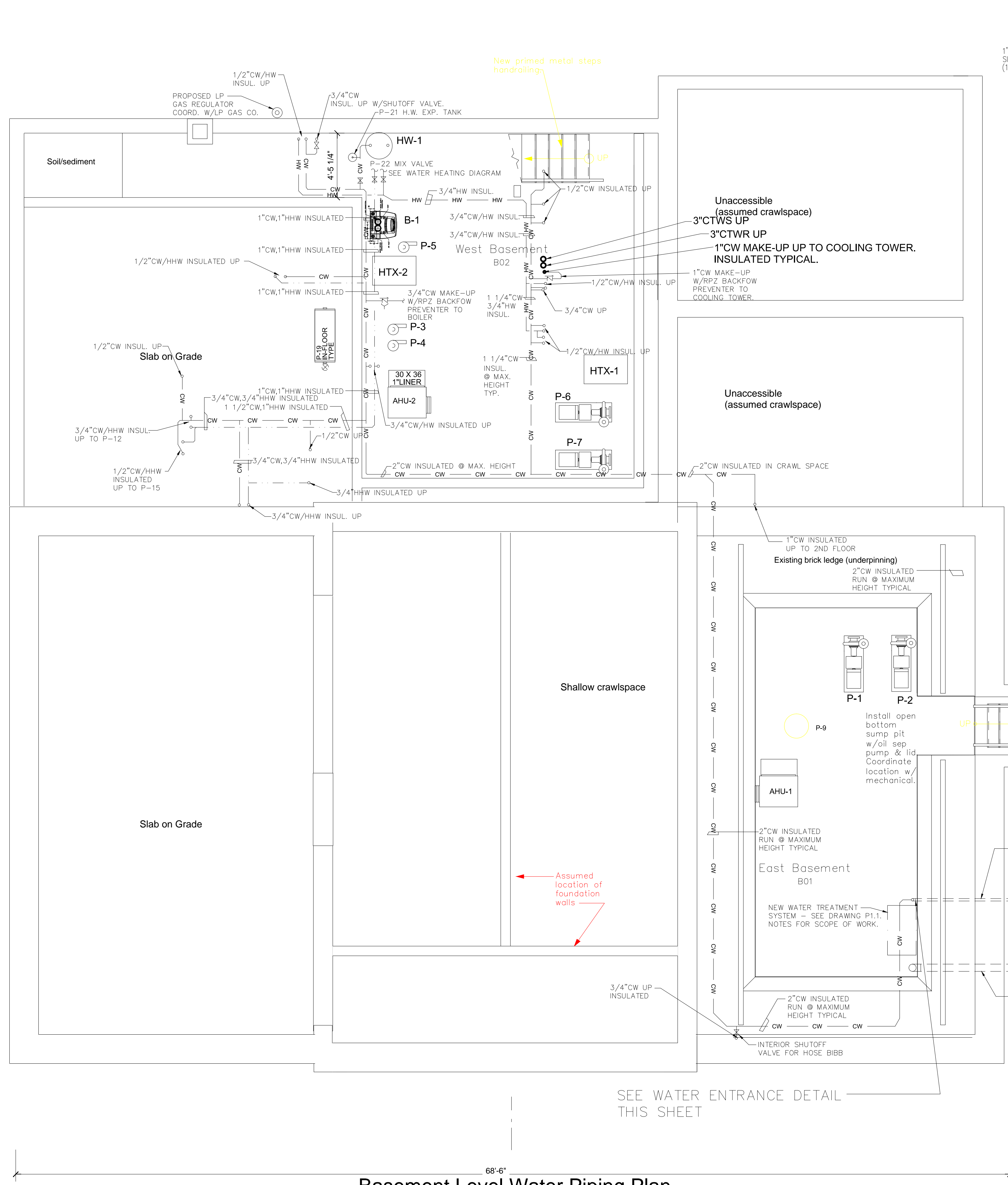
Basement Level Water Piping Plan Scale: 1/4" = 1'0"
