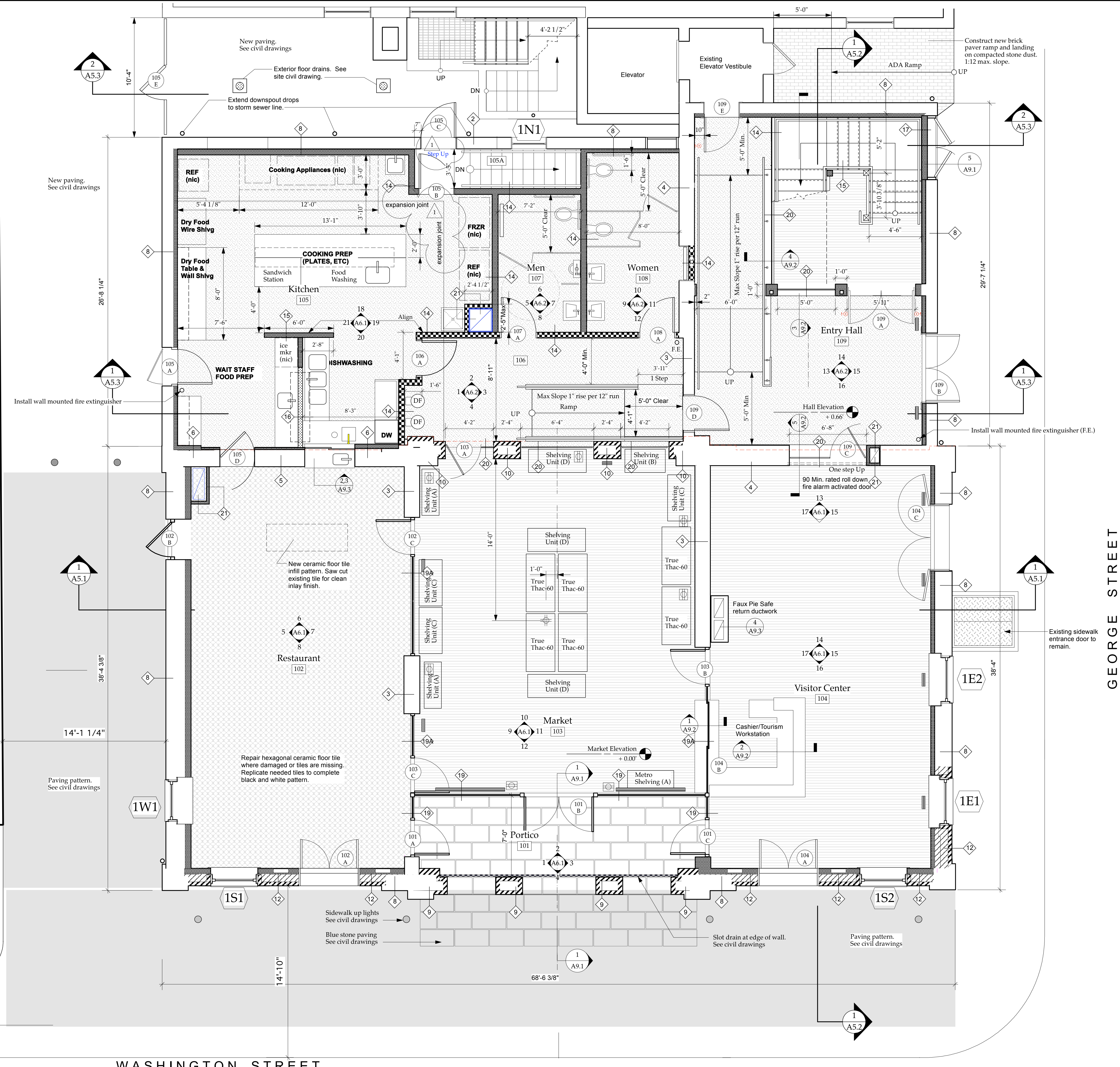
1 First Floor Plan Scale: 1/4" = 1'-0"
