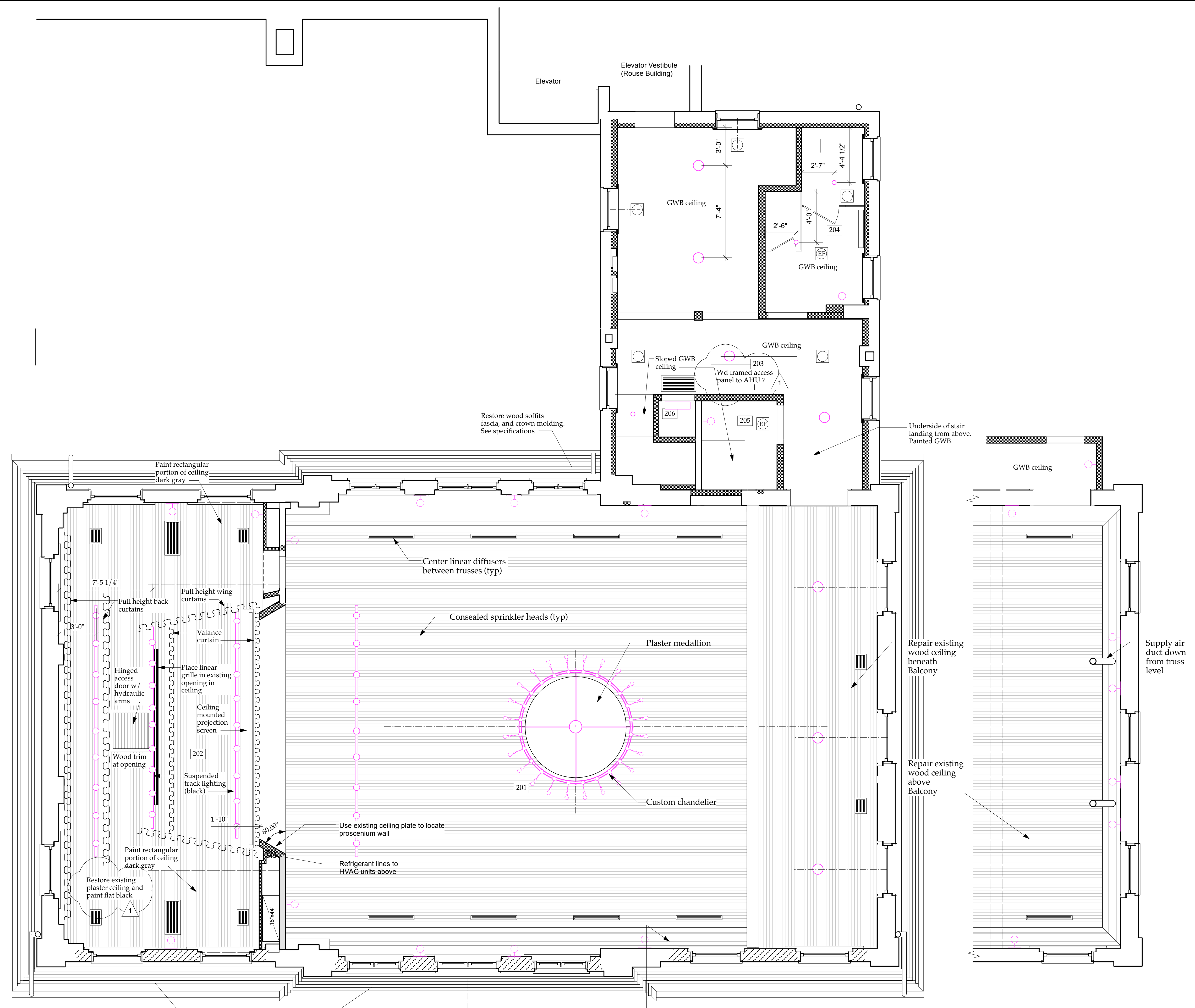
1 Balcony Level Scale: 1/4" = 1'-0"
