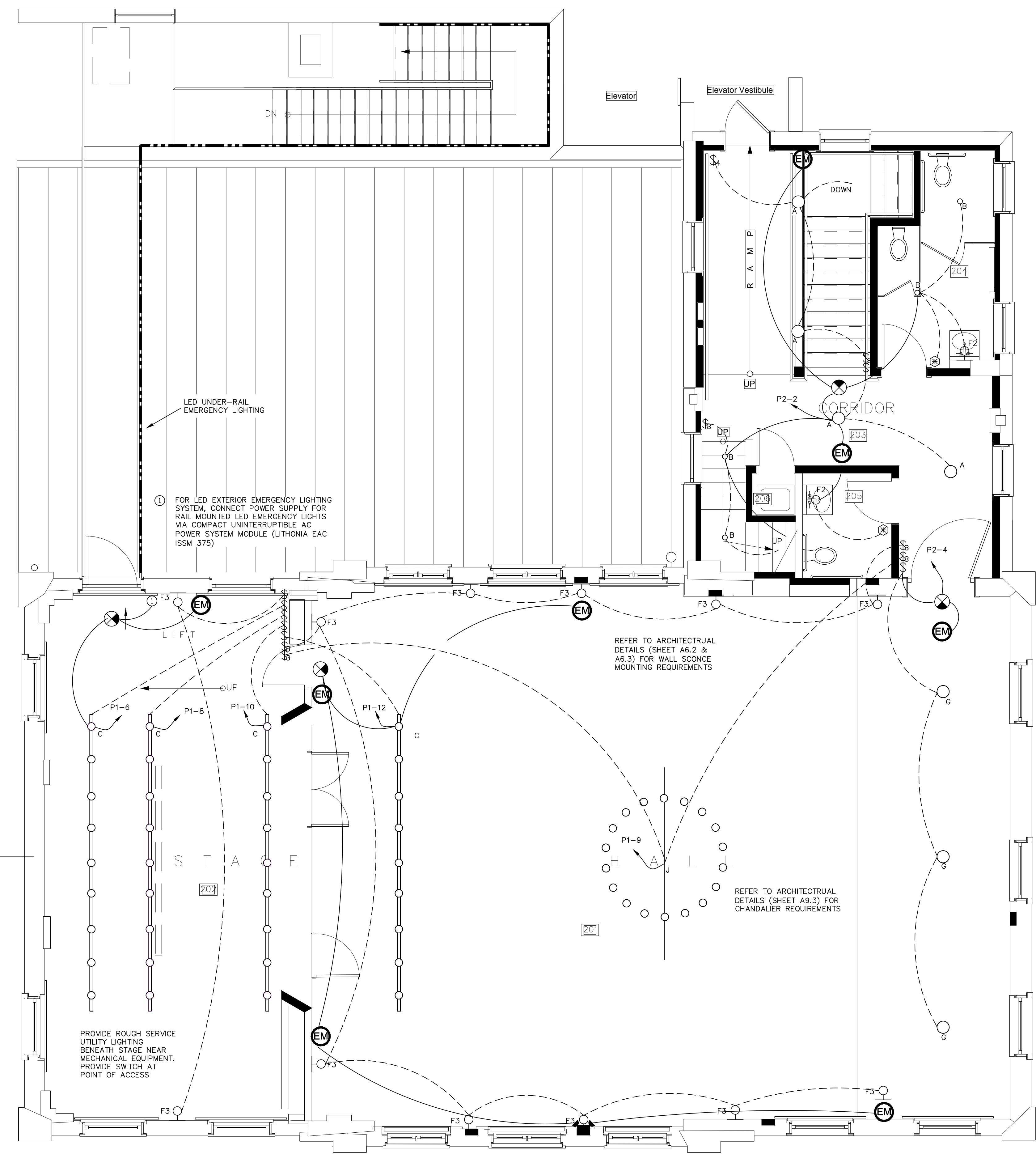
2ND FLOOR LIGHTING PLAN 1 E1-3 1/4" = 1'-0"
