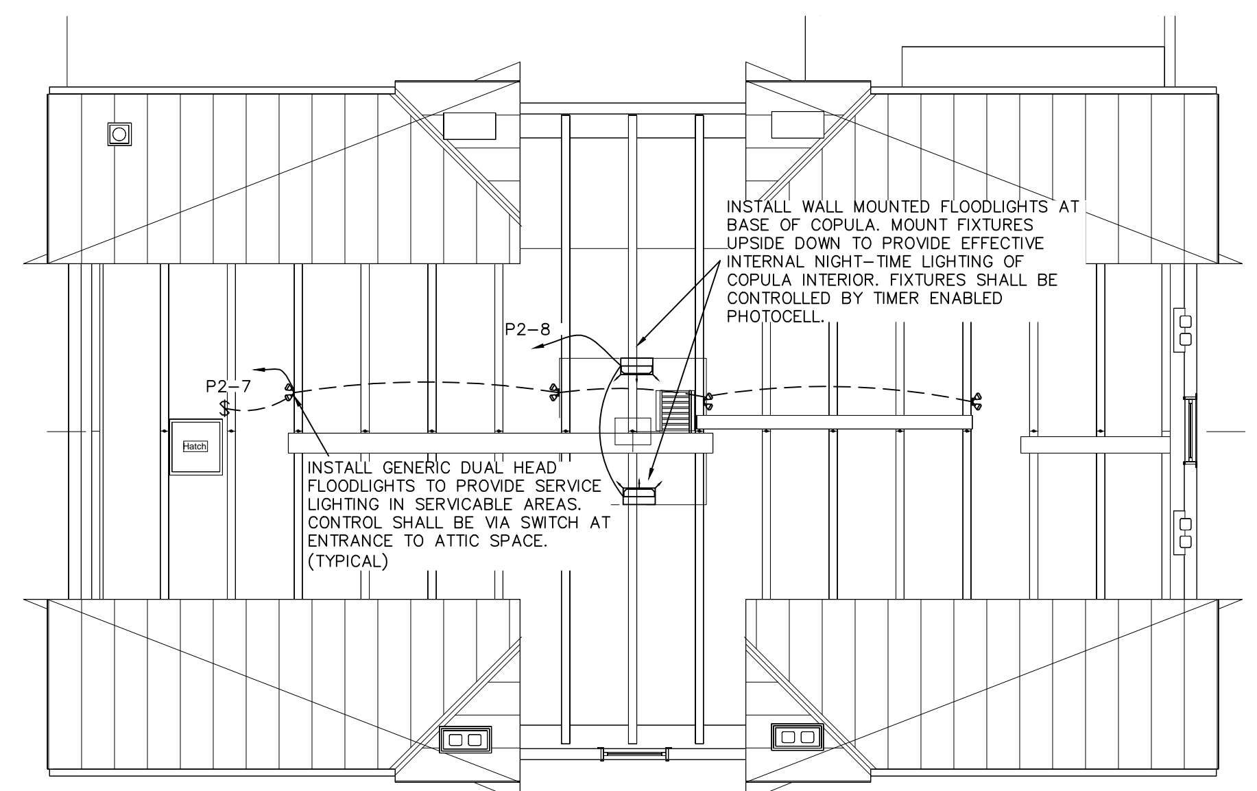
ATTIC LEVEL LIGHTING PLAN 3 E1-3 1/8" = 1'-0"
