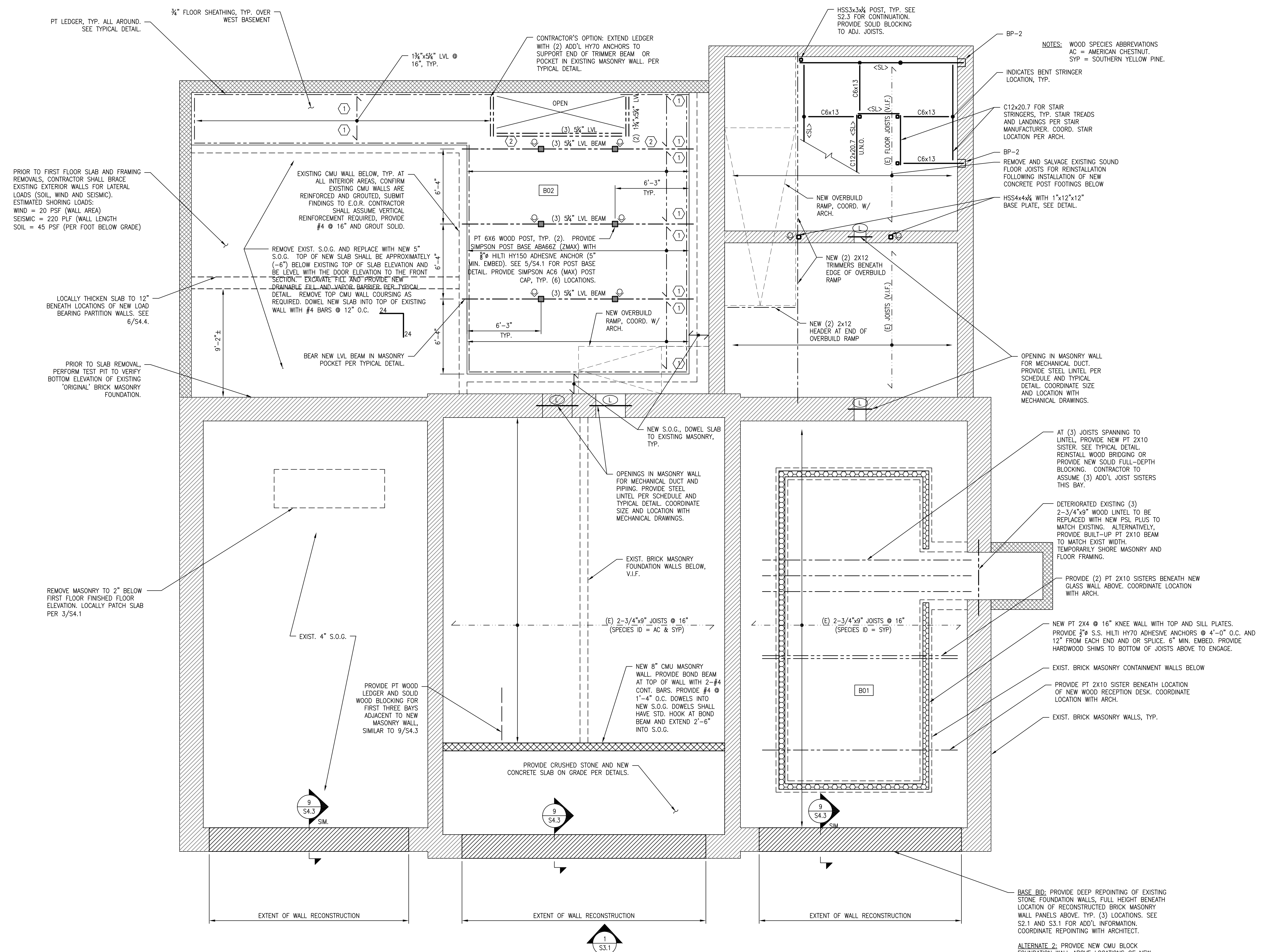
FIRST FLOOR FRAMING ON BASEMENT PLAN SCALE: 1/4" = 1'-0"
