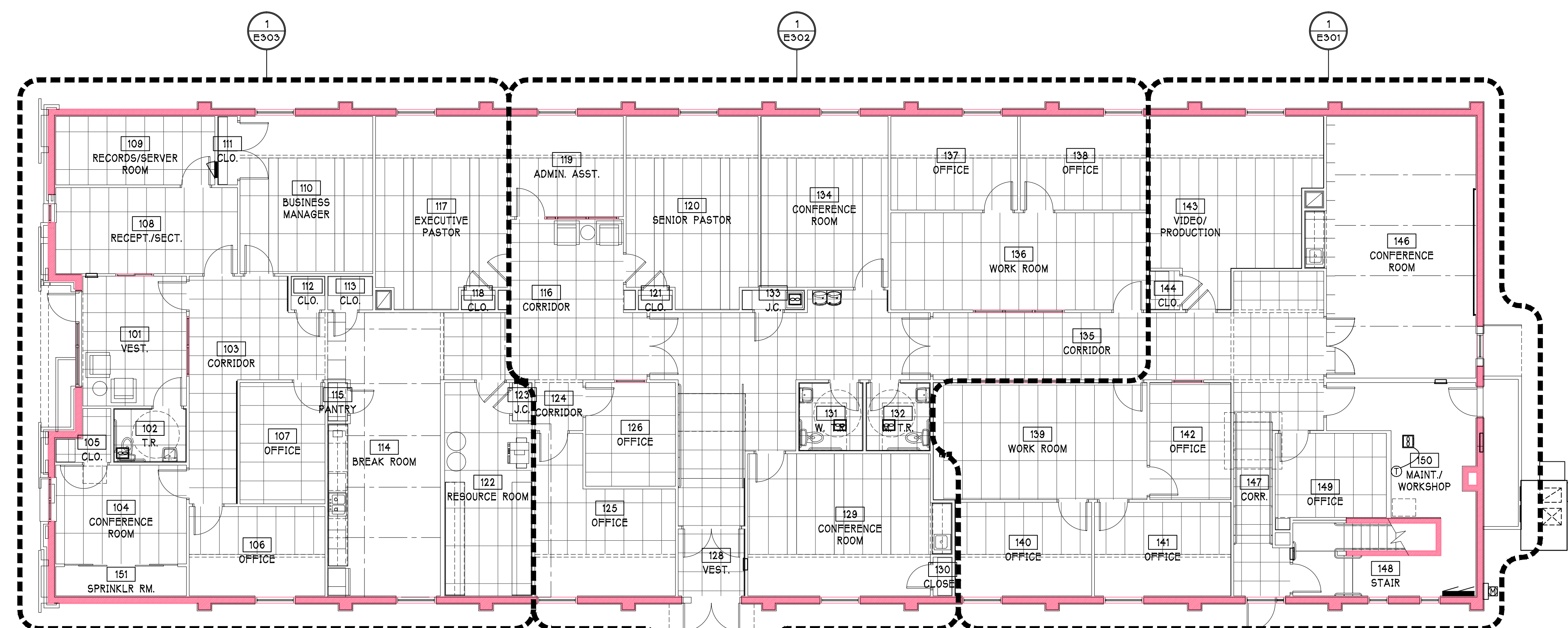
LIGHTING PLAN 1/8" = 1'-0"
